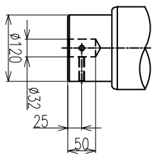
SHANK HOLE
