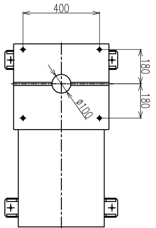
BOLSTER DIMENSION
