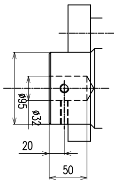
SHANK HOLE
