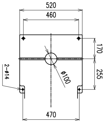
BOLSTER DIMENSION
