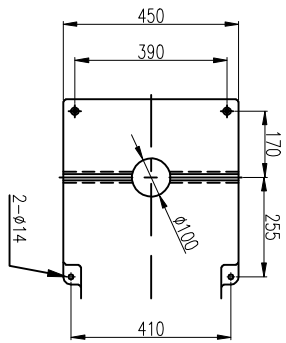
BOLSTER DIMENSION
