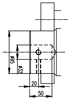
SHANK HOLE
